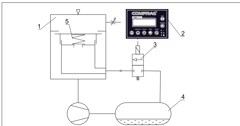
Fig. 2.5 Regulating system
